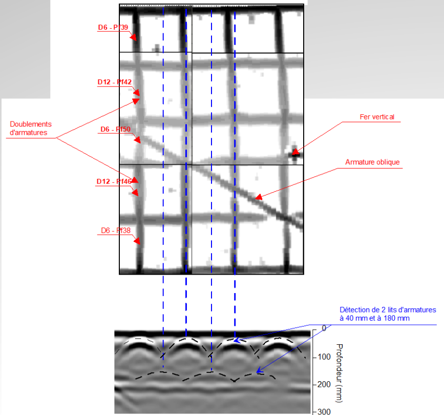
Radargramme
